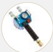
HAND-HELD DOUBLE DEADMAN CONTROLLER 8 bar (116 psi) 1.6 kg (3.5 lbs) 519820
